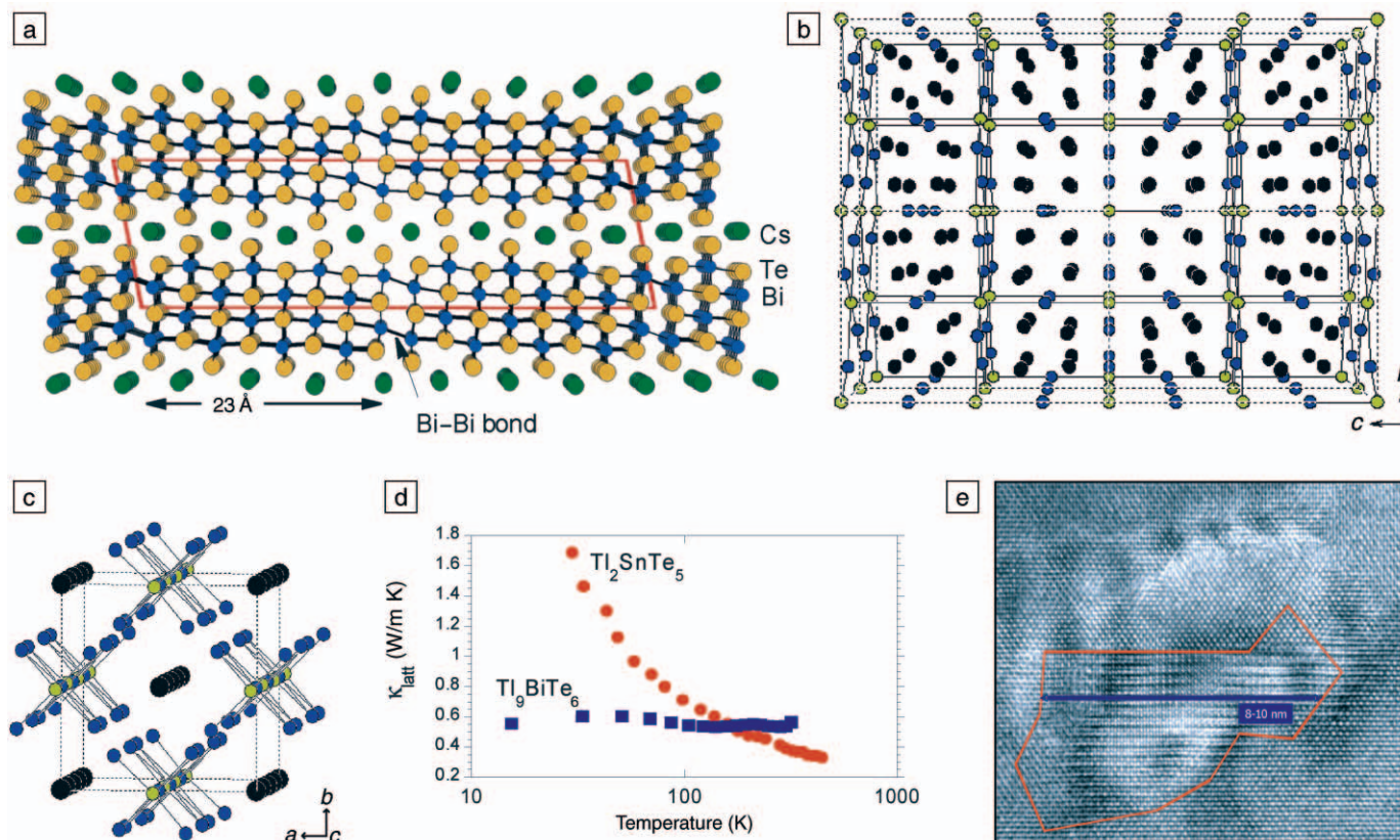
Figure 5. (a) Structure of CsBi 4 Te 6 . Yellow circles are Te atoms, blue circles are Bi atoms, and green circles are Cs atoms. (b) Structure of Tl 9 BiTe 6 . Yellow circles are Bi atoms, blue are Te atoms, and black are Tl atoms. (c) Structure of Tl 2 SnTe 5 . Black circles are Tl atoms, blue are Te atoms, and yellow are Sn atoms. (d) Thermal conductivity of Tl 9 BiTe 6 and Tl 2 SnTe 5 . (e) High-resolution transmission electron microscopy image of a typical nanoscale inhomogeneity (indicated by the red outline) found in Ag 1-x Pb 18 SbTe 20 .
